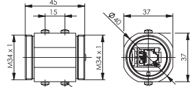
TOC coupler
